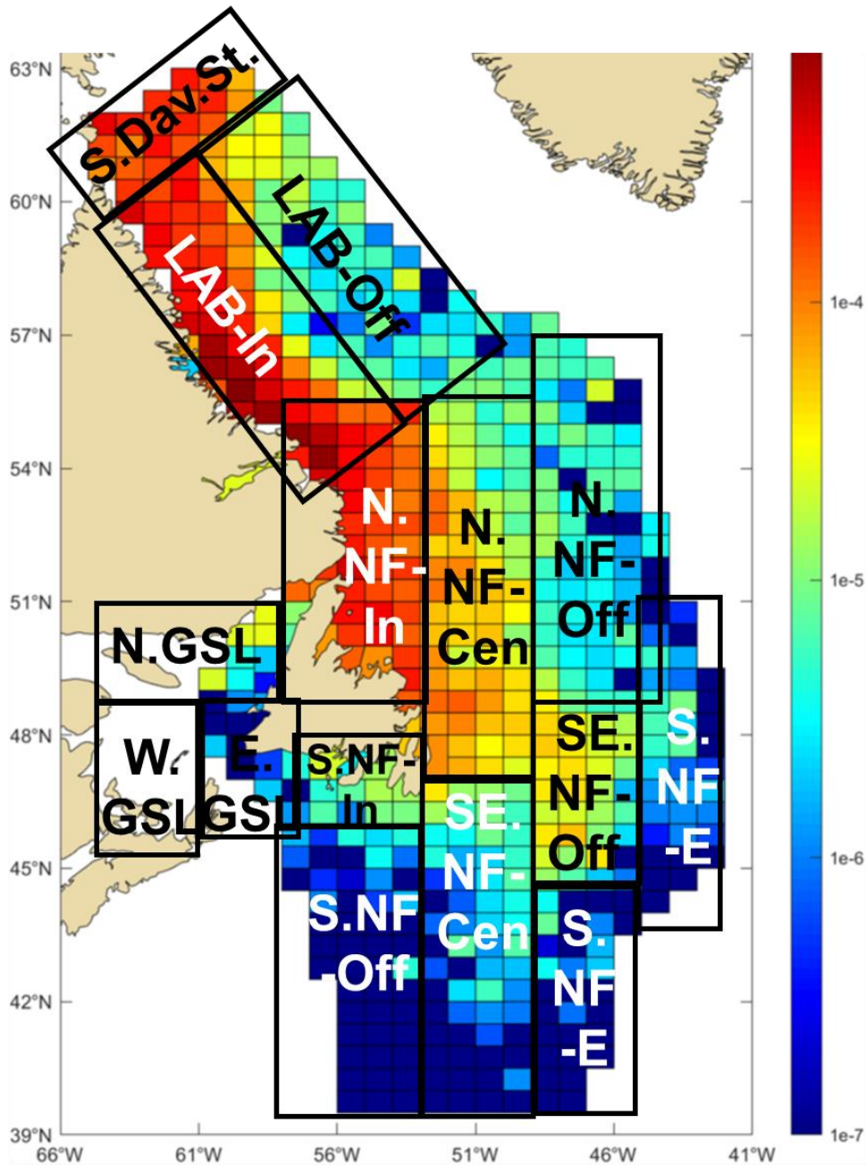
Figure 3-20 - Different regions of iceberg densities (km 2 ) in Atlantic Canada waters (C-CORE, 2017).
